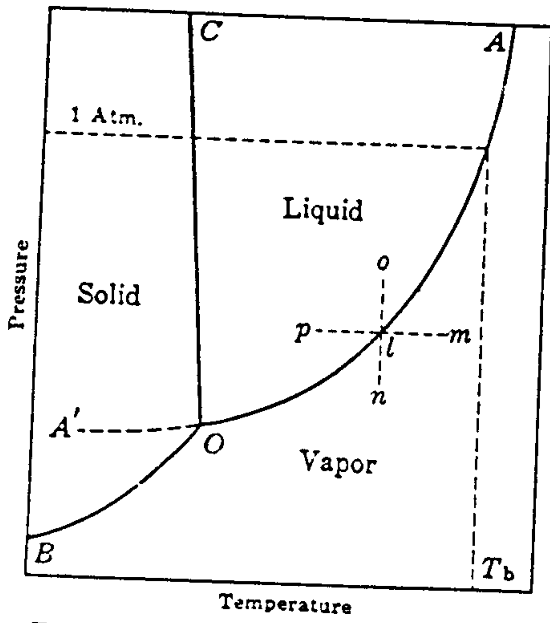
FIG. 99. Solid-liquid-vapor equilibria
