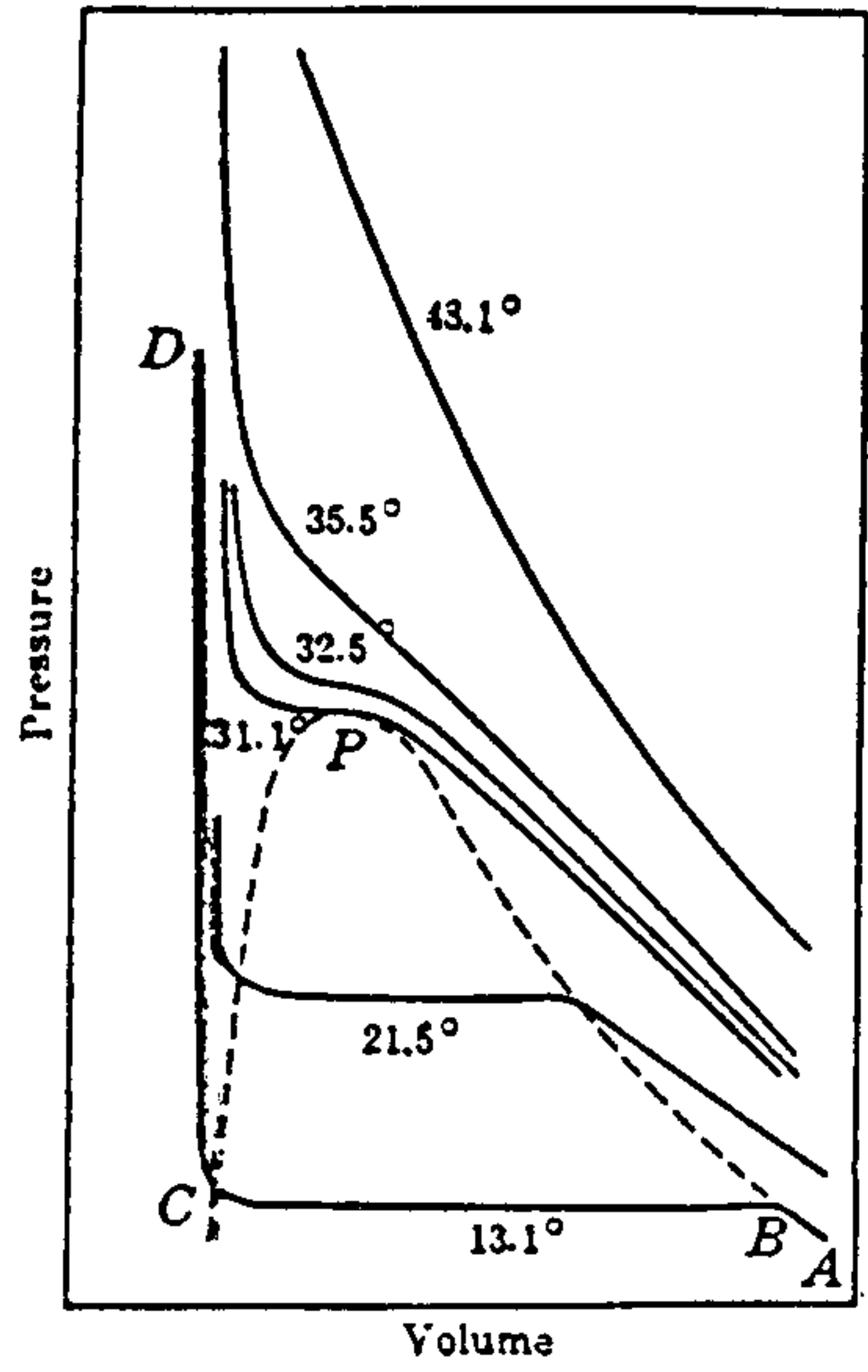
FIG. 91. Pressure-volume curves of carbon dioxide
