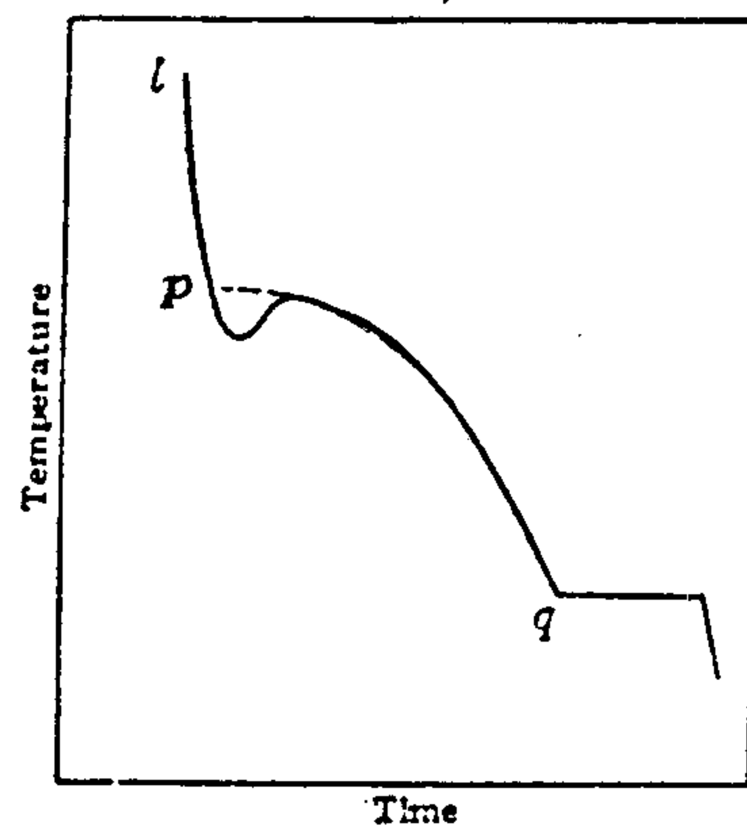
Fig. 175. Cooling curve with supercooling
